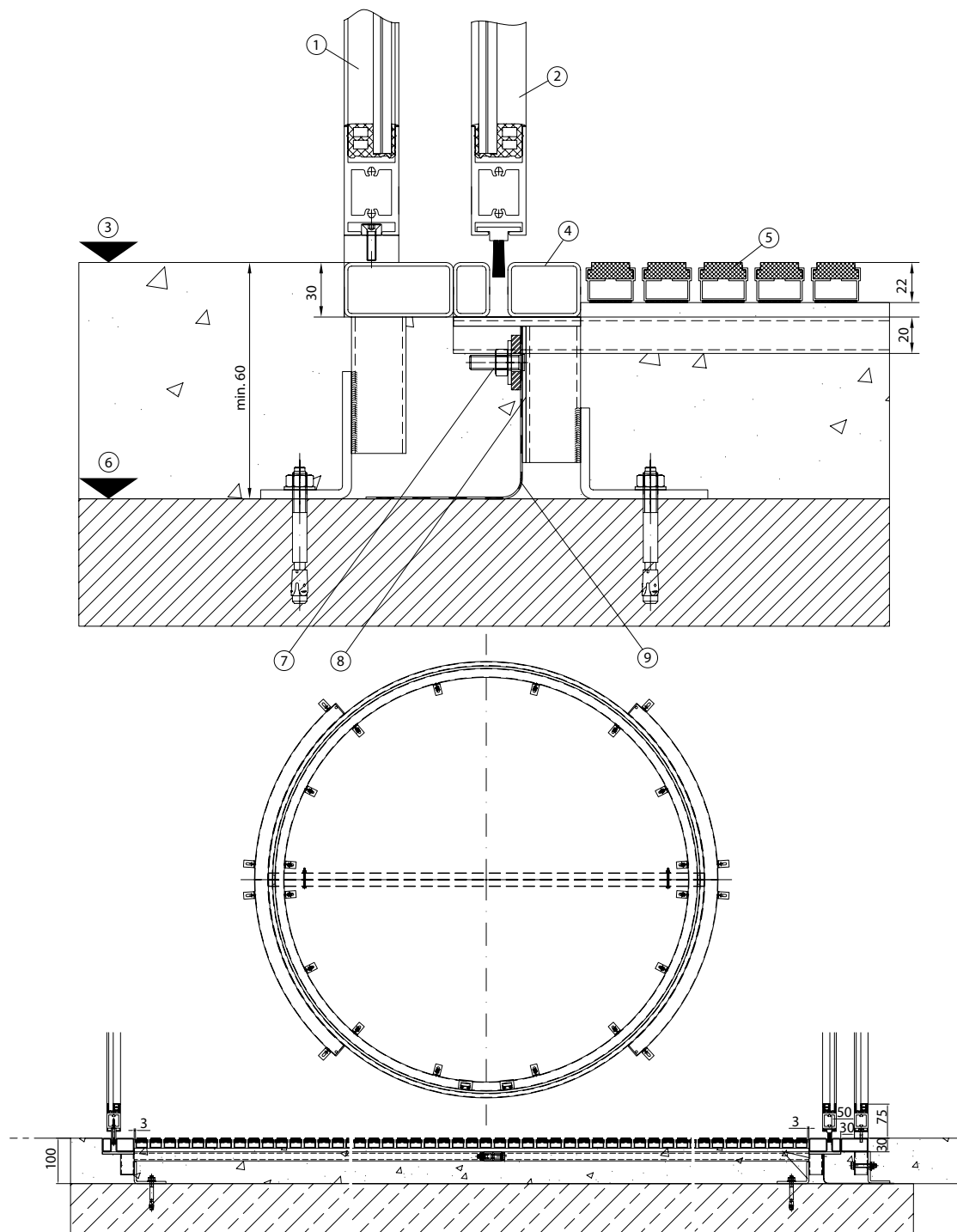
Floor ring
