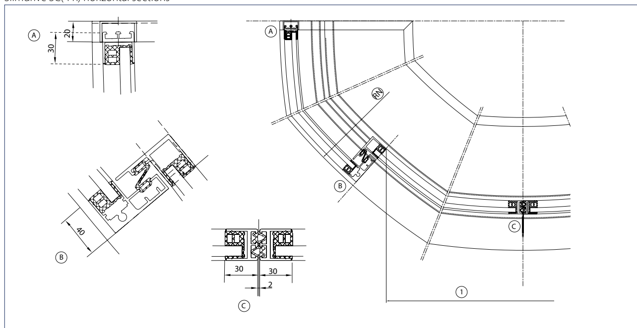
Slimdrive SC(-FR) horizontal sections
